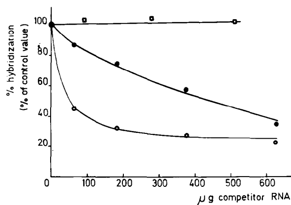
Fig.1. Competition hybridization between RNA synthesized in vitro on \phi 80d argECBH ppc DNA and RNA isolated from E. coli K 12 P4XB2 and E. coli K12 MN42. 0.08 \mu g of ^3H -labelled RNA synthesized in vitro ( 1.25 \times 10^5 cpm) was hybridized with 0.11 \mu g of either light or heavy strands of \lambda 14 DNA, in the presence of increasing amounts of unlabelled competitor RNA (circles = P4XB2 ; squares = MN42). Hybridization efficiency in the absence of competitor RNA, which represents the 100% value of the control is about 50% of that observed with a large excess of separated strands of \lambda 14 DNA. Background, mock hybridizations performed at 0°C, were subtracted from all values. (○—○—○) hybridization with the heavy strand of \lambda 14 DNA; (●—●—●) hybridization with the light strand of \lambda 14 DNA; (□—□—□) hybridization with heavy strand of \lambda 14 DNA.
